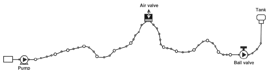
FIGURE 10 Pipeline schematic example 2
