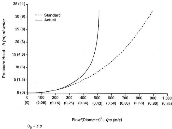
FIGURE 1 Flow of air through an orifice
