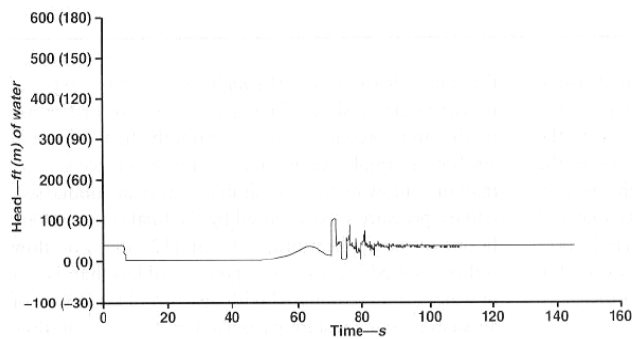
FIGURE 12 Surge analysis for example 2, 1-in. (25-mm) orifice
