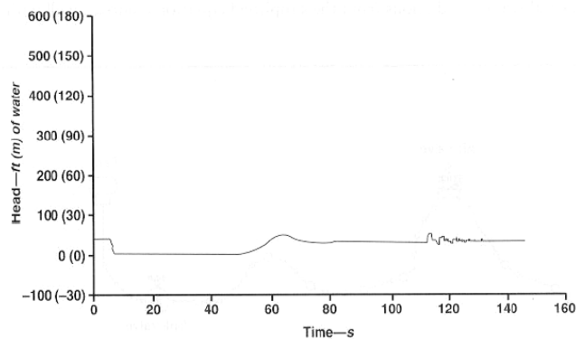
FIGURE 13 Surge analysis for example 2, 0.5-in. (12.5-mm) orifice
