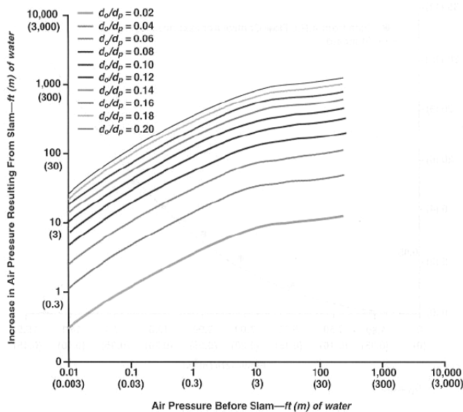
FIGURE 4 Air-slam pressures for different outlet orifice sizes
