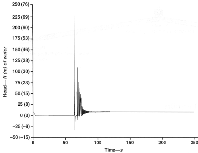
FIGURE 8 Surge analysis for a 1-in. (25-mm) orifice
