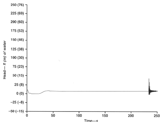
FIGURE 9 Surge analysis for a 0.5-in. (12.5-mm) orifice
