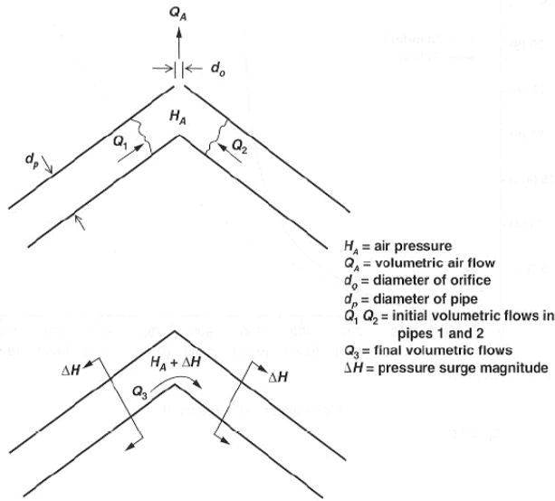
FIGURE 3 Conditions before and after an air slam
