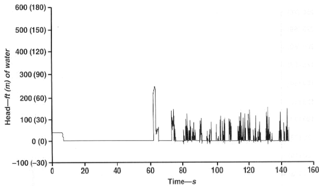
FIGURE 11 Surge analysis for example 2, 3-in. (75-mm) orifice
