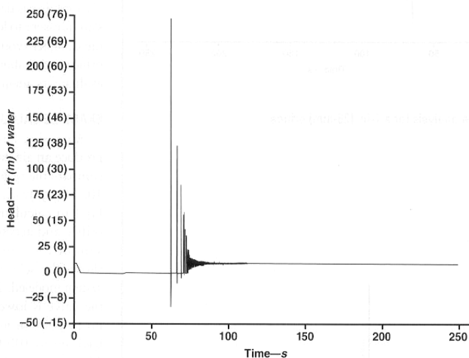
FIGURE 6 Surge analysis for a 4-in. (100-mm) orifice
