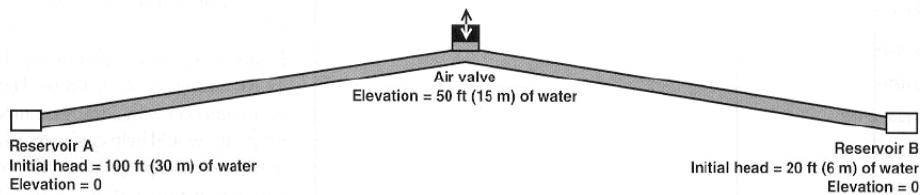
FIGURE 5 Transient flow model to calculate air slam
